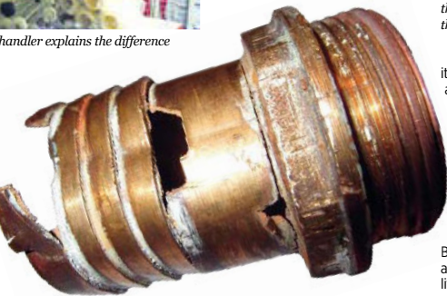
An ordinary brass tailpipe found during the survey of a 10-year-old boat. It was so badly dezincified that the wall simply crumbled under a light tap. The tailpipe was on a cockpit drain always left open. Left like this, it would only be a matter of time before the boat sank.
